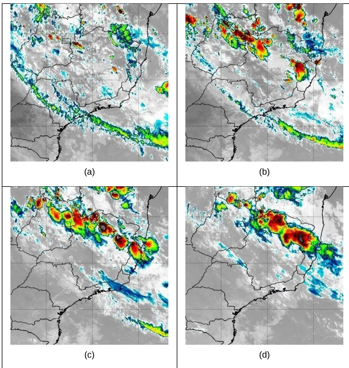
Figura 9 Imagens de Satélite do dia 22/10 as 13:00 (a), 16:00 (b), 19:00 (c) e 22:00 (d)
