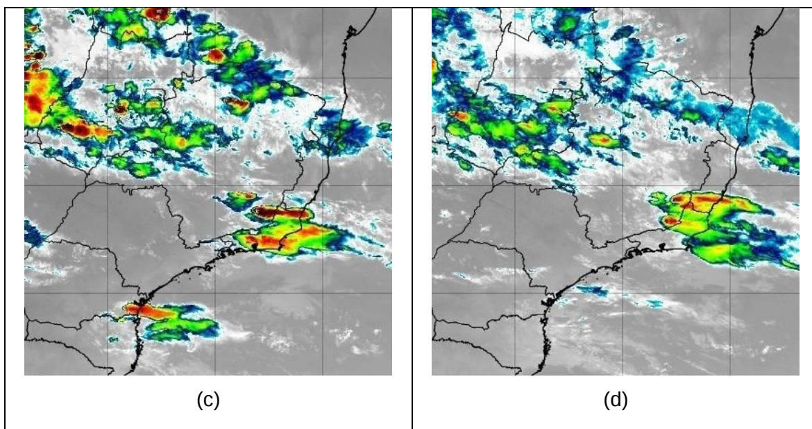
Figura 7 Imagens de Satélite do dia 25/10 as 13:00 (a), 16:00 (b), 19:00 (c) e 22:00 (d).
