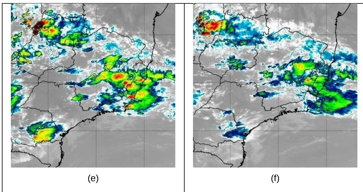
Figura 12 Imagens de Satélite do dia 26/10 as 07:00 (a), 10:00 (b), 13:00 (c), 16:00 (d), 19:00 (c) e 22:00 (d). Fonte INPE.
