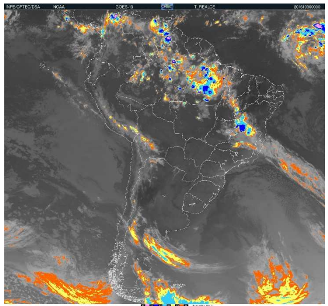
Dia 30/10 00:00h UTC
