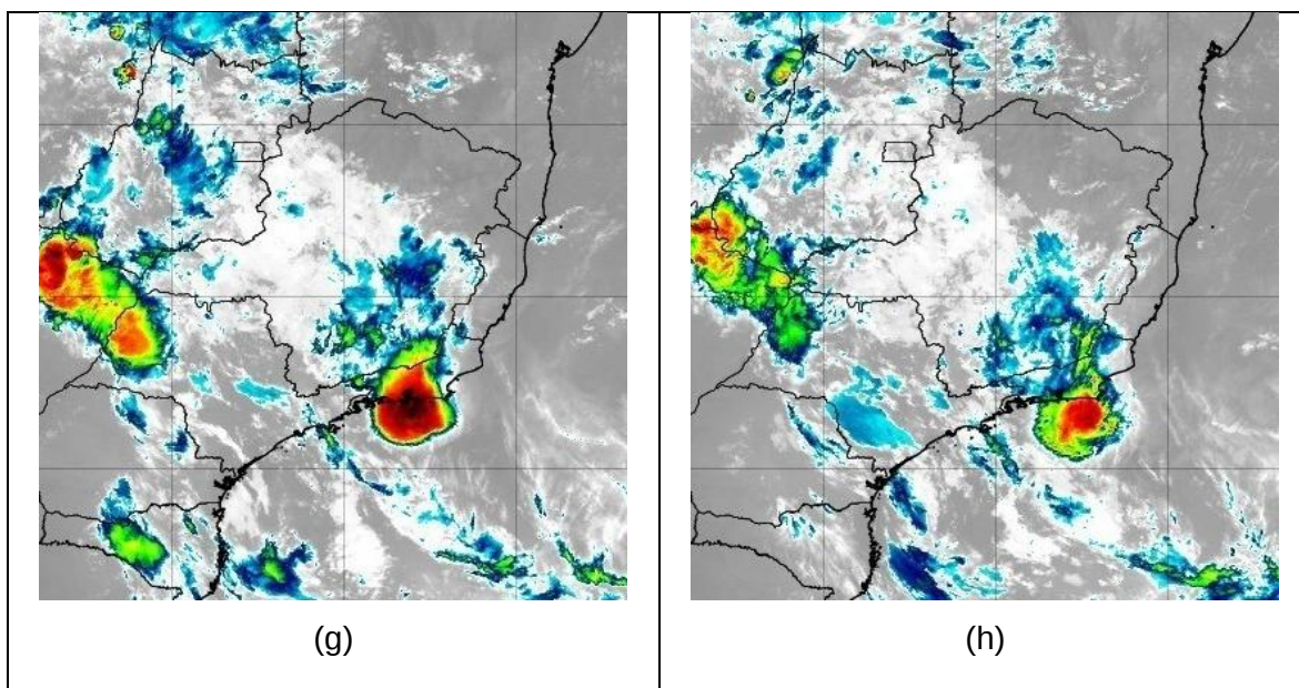
Figura 3 Imagens de Satélite do dia 27/10 as 21:00 (a) e do dia 28/10 as 03:00 (b), 09:00 (c), 15:00 (d), 17:00 (e), 19:00 (f), 21:00 (g) e 23:00 (h)
