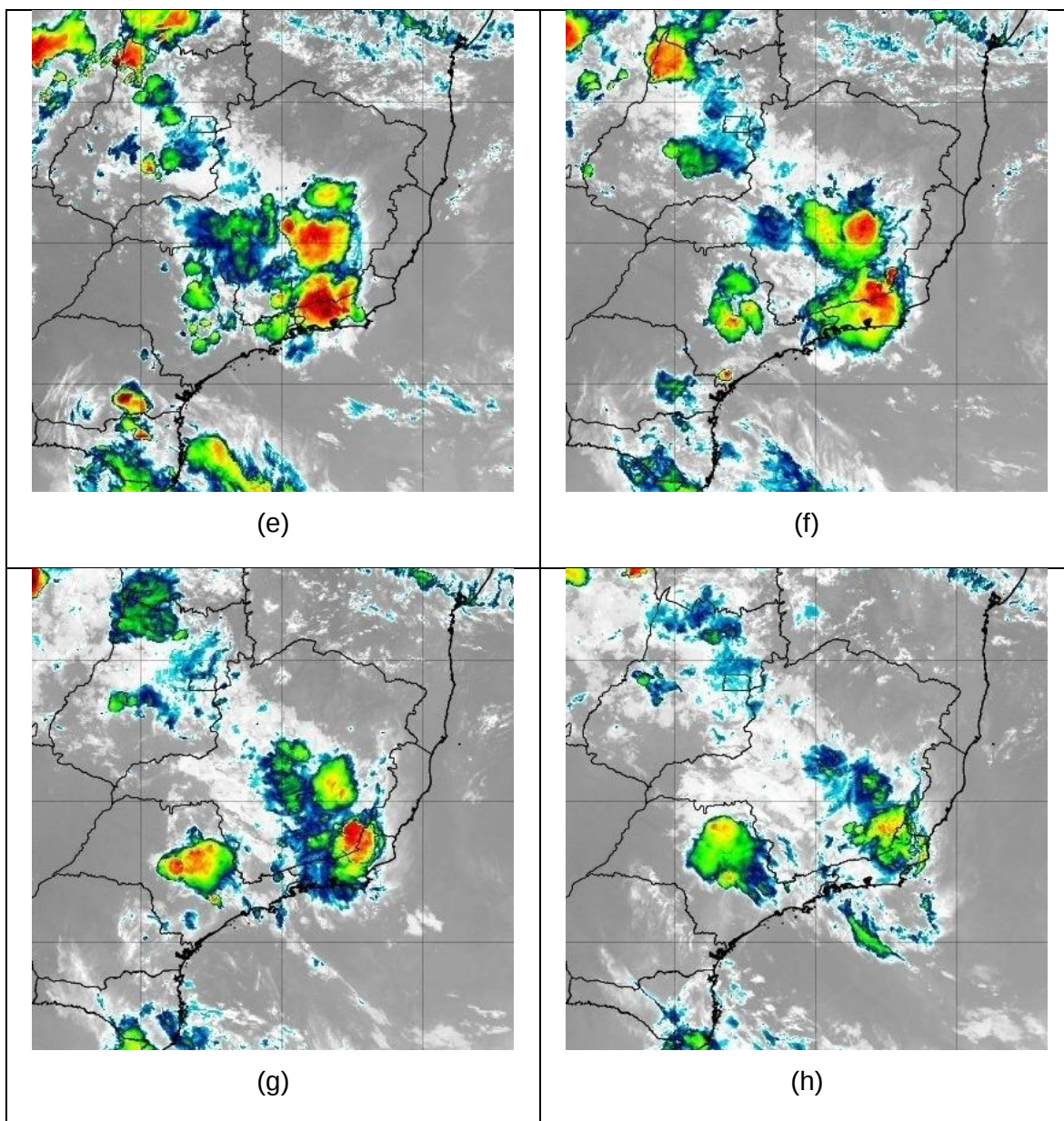
Figura 7 Imagens de Satélite do dia 29/10 as 10:00 (a), 12:00 (b), 14:00 (c), 16:00 (d), 18:00 (e), 20:00 (f), 22:00 e (g) 24:00 (h)
