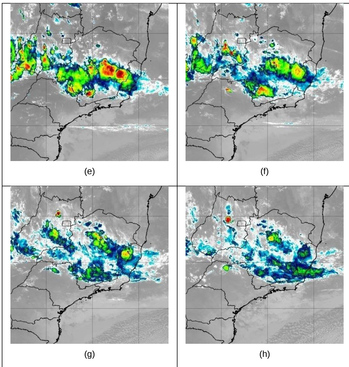
Figura 19 Imagens de Satélite do dia 01/11 as 10:00 (a), 12:00 (b), 14:00 (c), 16:00 (d), 18:00 (e), 20:00 (f), 22:00 (g) e 24:00 (h)
