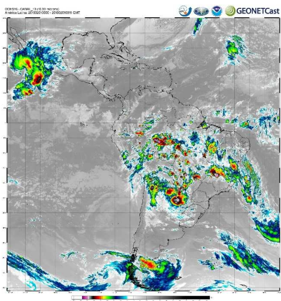
Dia 01/02 00:00 UTC
