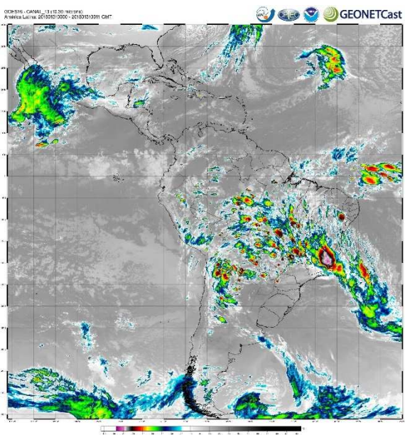
Dia 31/01 00:00 UTC
