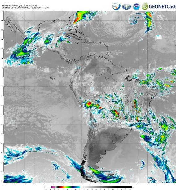
Dia 29/01 21:00 UTC
